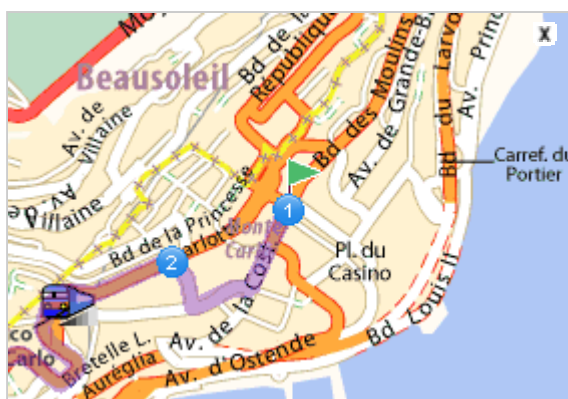
Departure: 98000 Monte-Carlo
